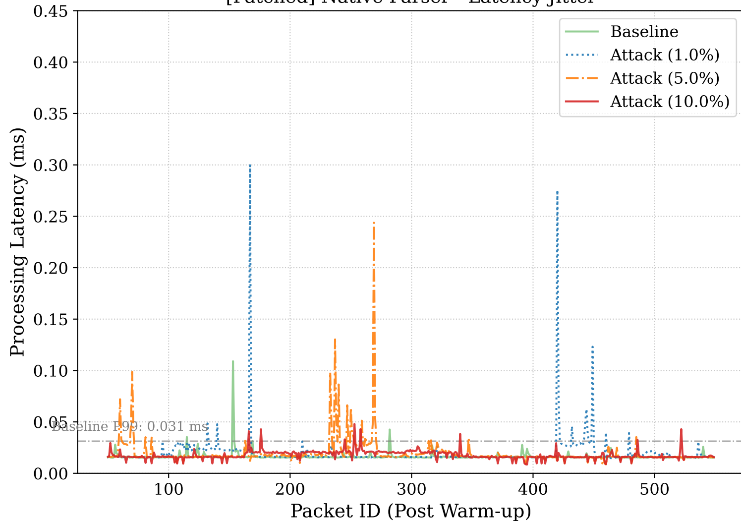
[Patched] Native Parser - Latency Jitter
