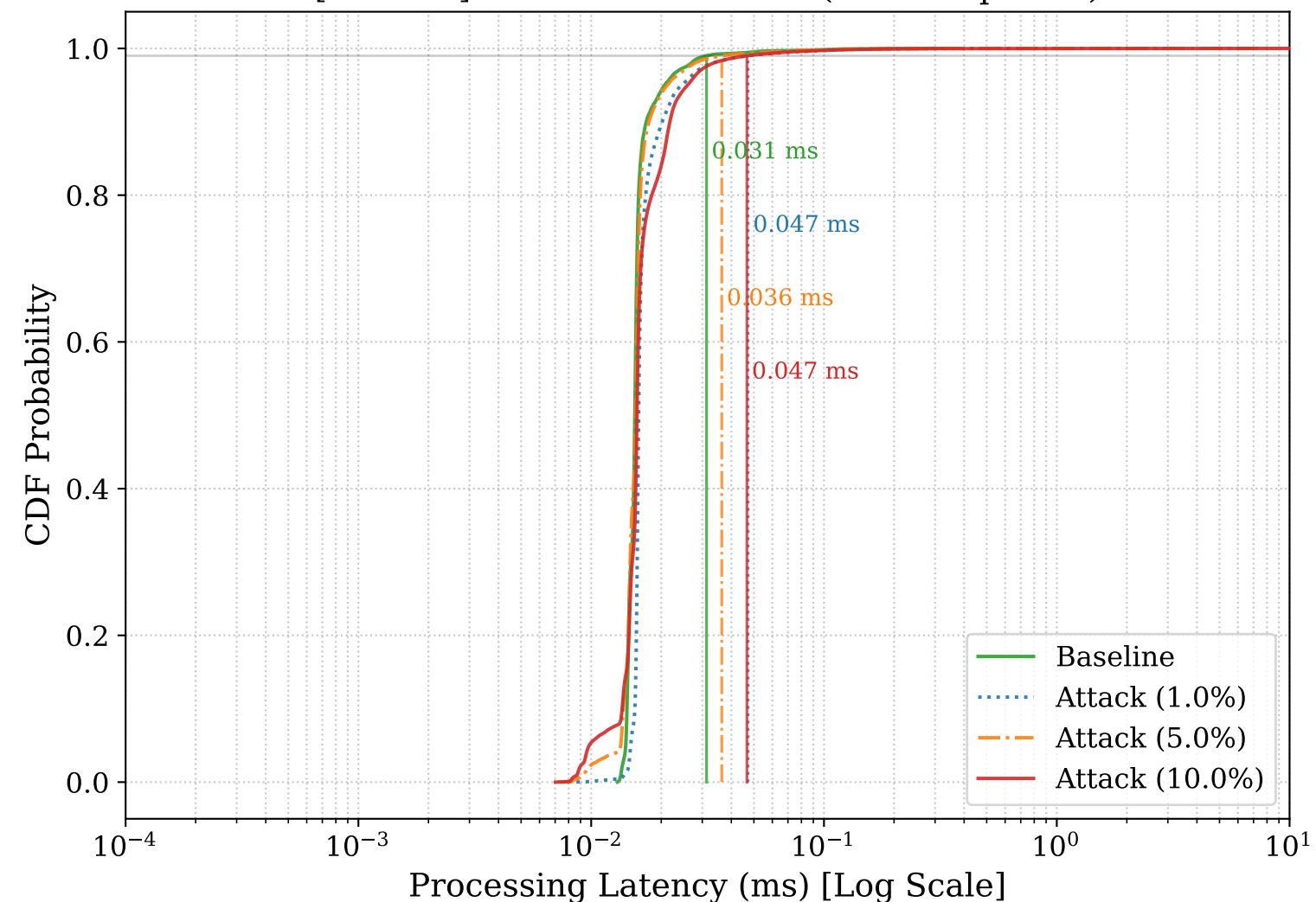
[Patched] Native Parser - CDF (99th Drop-lines)
